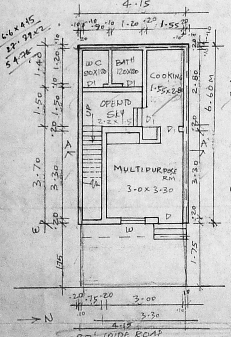
LOCATION & GROUND FLOOR PLAN (EXG. BLDG. CONSTRUCTED BY TNHB)
